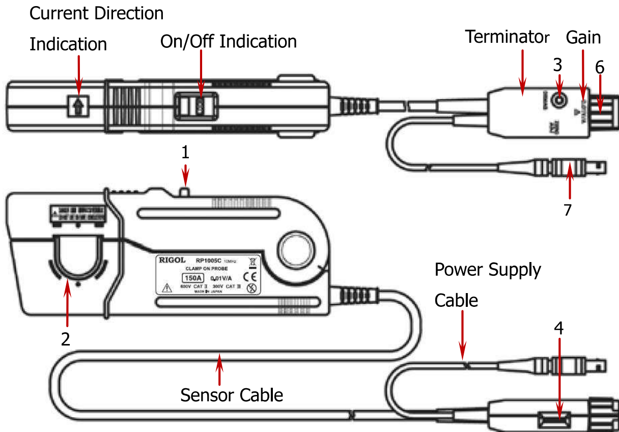
Figure 3 RP1005C Parts
