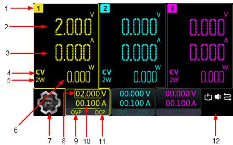
Figure 4.6 User Interface
